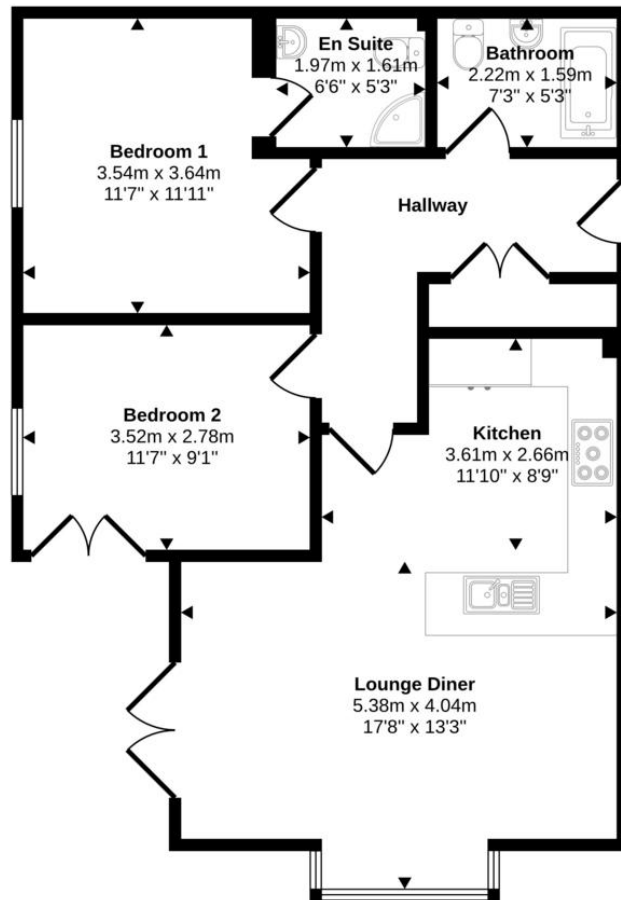
Floorplan
